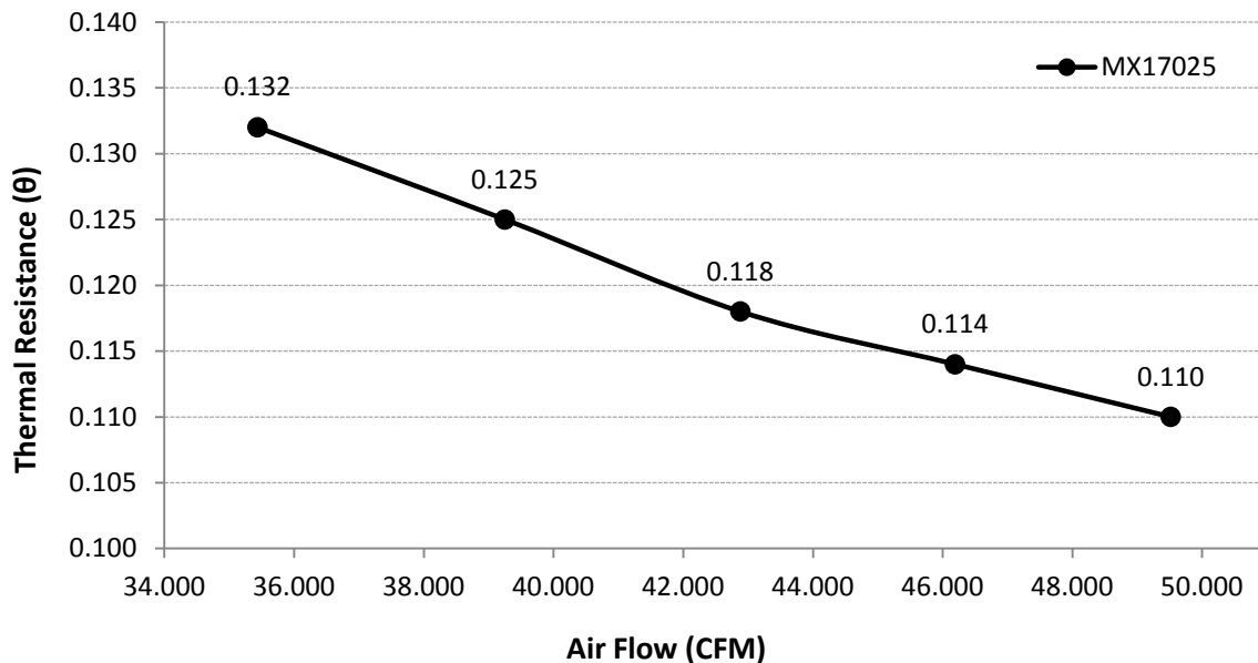
Test Power: 240W Heater Dimension :47*70mm
